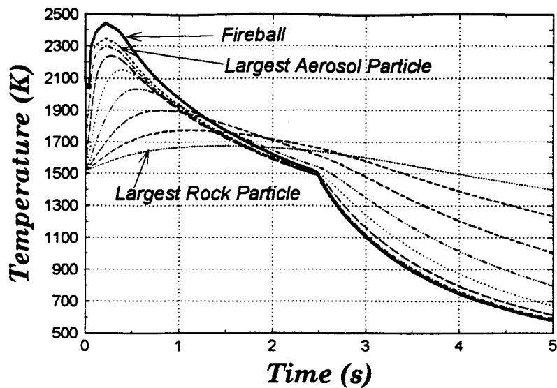
Figure 9. Particle Temperature Response
