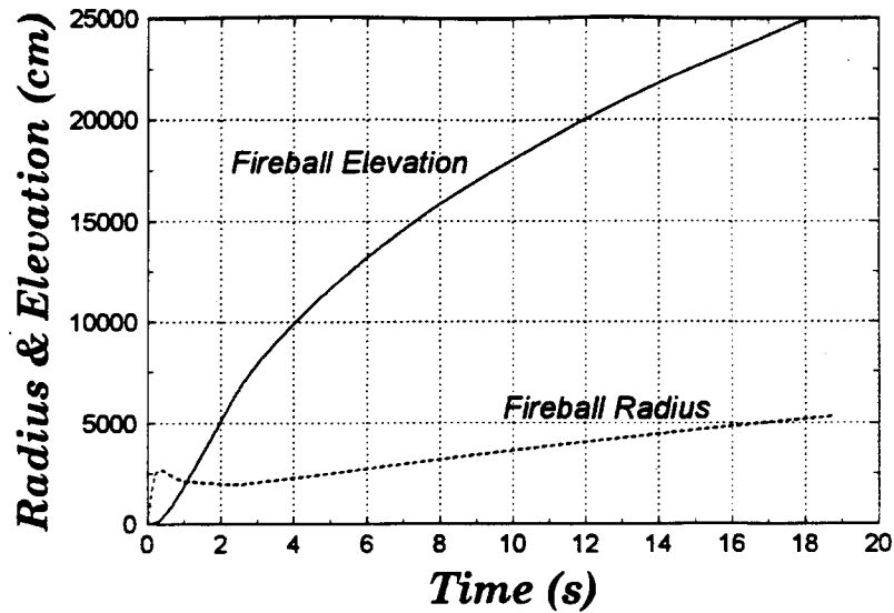
Figure 7. Fireball Radius and Elevation
