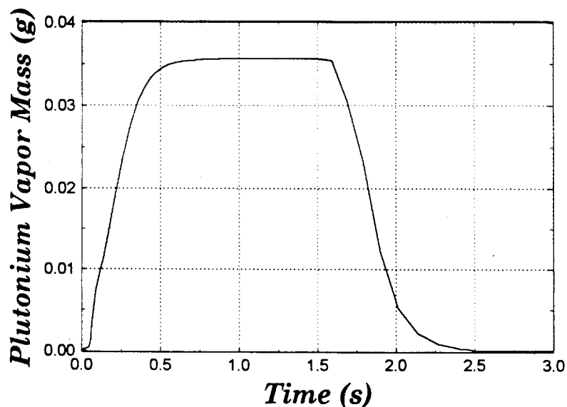
Figure 10. Plutonium Vapor Mass in the Fireball
