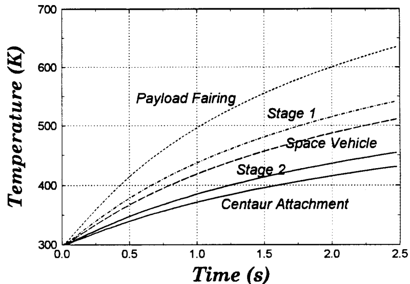
Figure 8. Aluminum-Alloy Structure Temperatures
